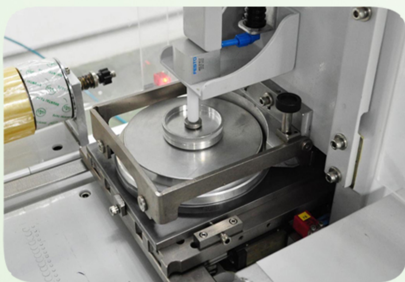
Ø165mm sealed ink cup (Wide coverage)
