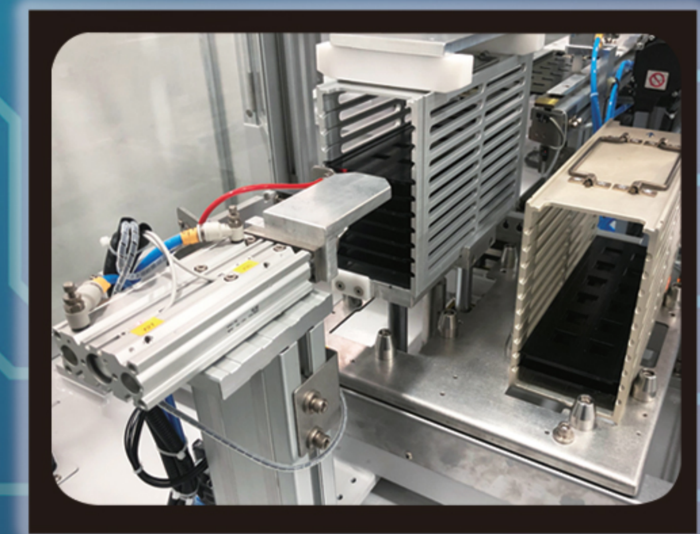
Load / unload I.C. cartridge
